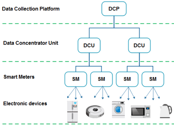
Fig. 2: Hierarchical organization of AMI components
