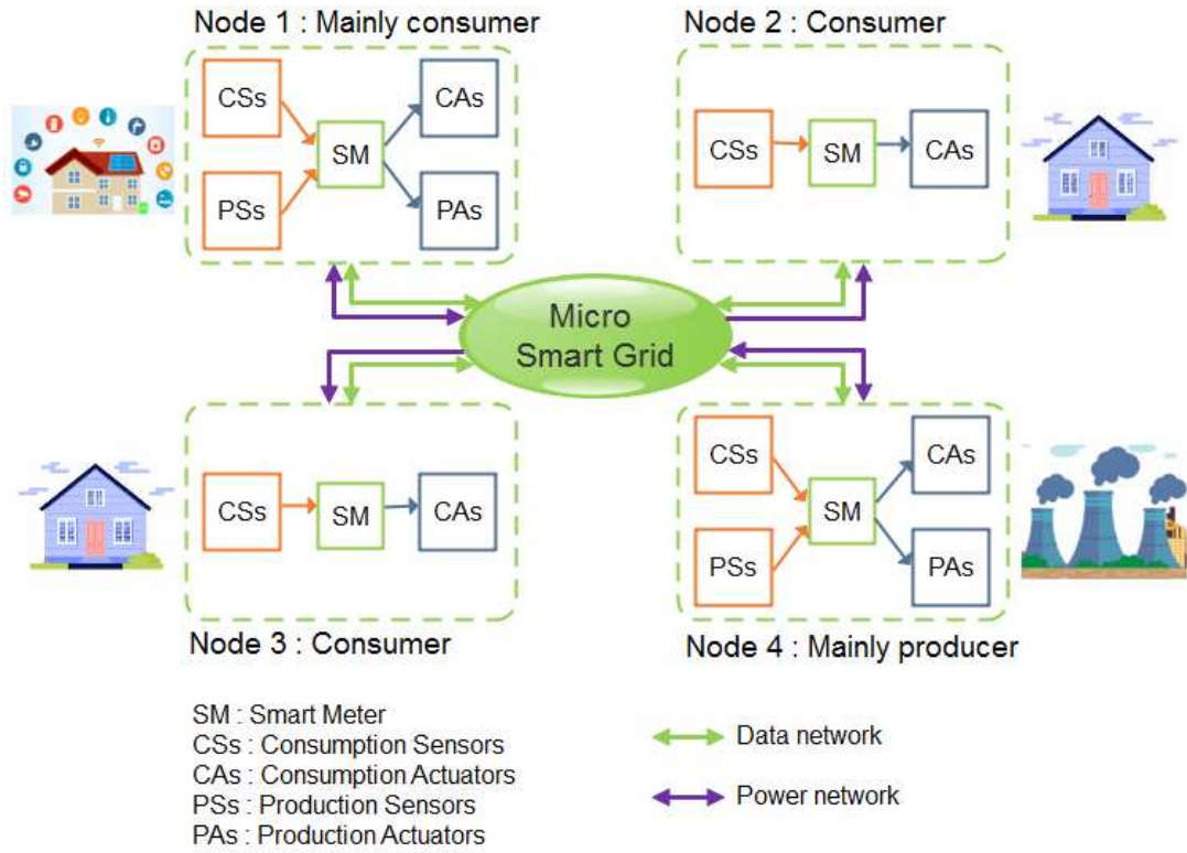
Fig. 3: Micro Smart Grid model according to the ReDy architecture
