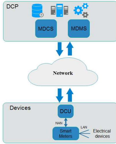
Fig. 1: AMI systems description
